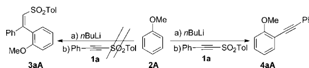
Scheme 2. Alkynylation of anisole with arylsulfonylacetylenes.
