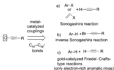
Scheme 1. Approaches for the synthesis of C sp –C sp 2 bonds.
